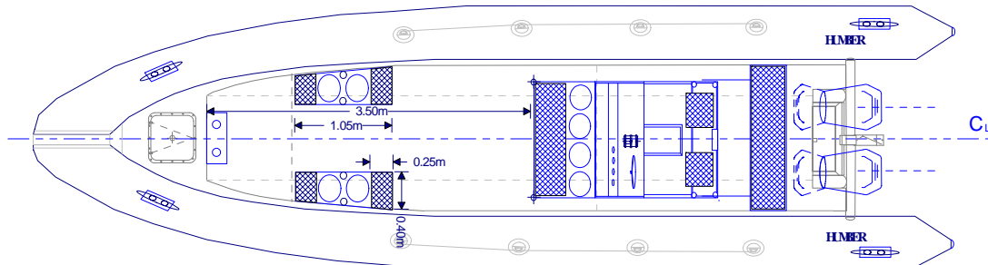
11m (3.3m beam) Cabin Windfarm RHIB
