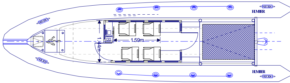
10m (2.8m beam) Cabin with single inboard
