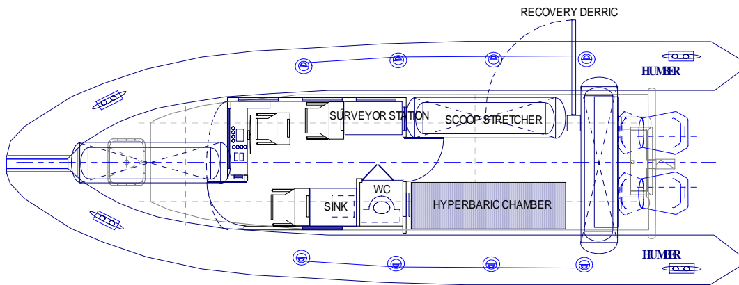
Cabin Dive Recovery RHIB
