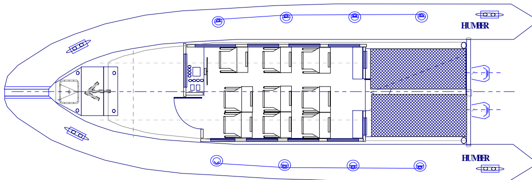
11m (3.3m beam) Cabin Windfarm RHIB
